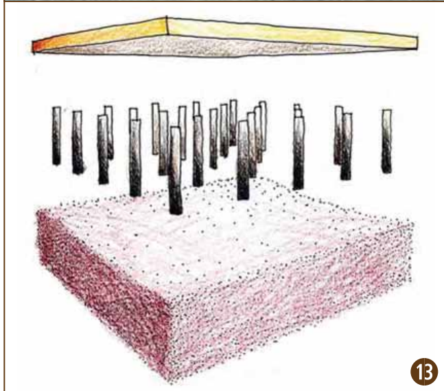
Figure 13 Suspending the sidewalk on vertical supports stabilizes the walk and allows roots to grow well in uncompacted soil.
